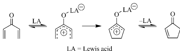
Figure 1. Nazarov cyclization pathway.
