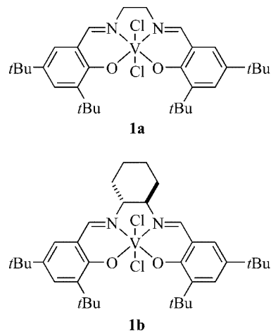
Figure 2. Vanadium salen complexes 1a and 1b .
