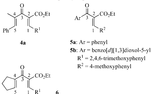
Figure 3. The types of dialkenyl ketones tested in this study.
