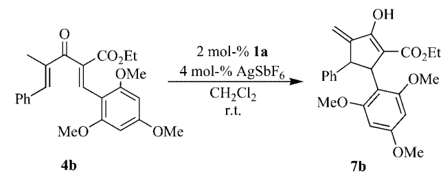
Scheme 1. Cyclization of 4b .
