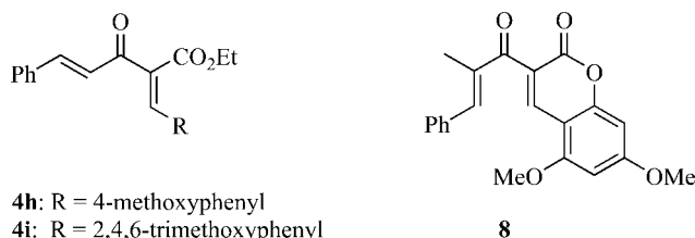
Figure 4. Conformations of divinyl ketones.
